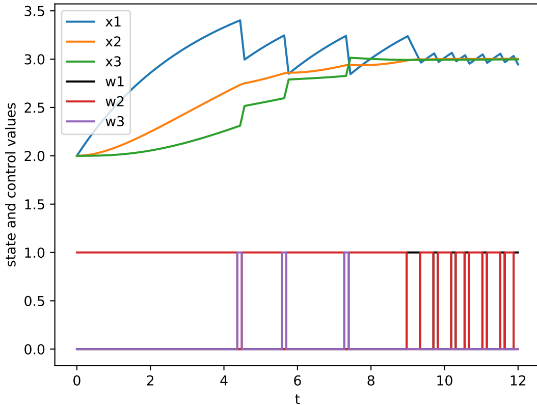
Differential state trajectories for binary controls
